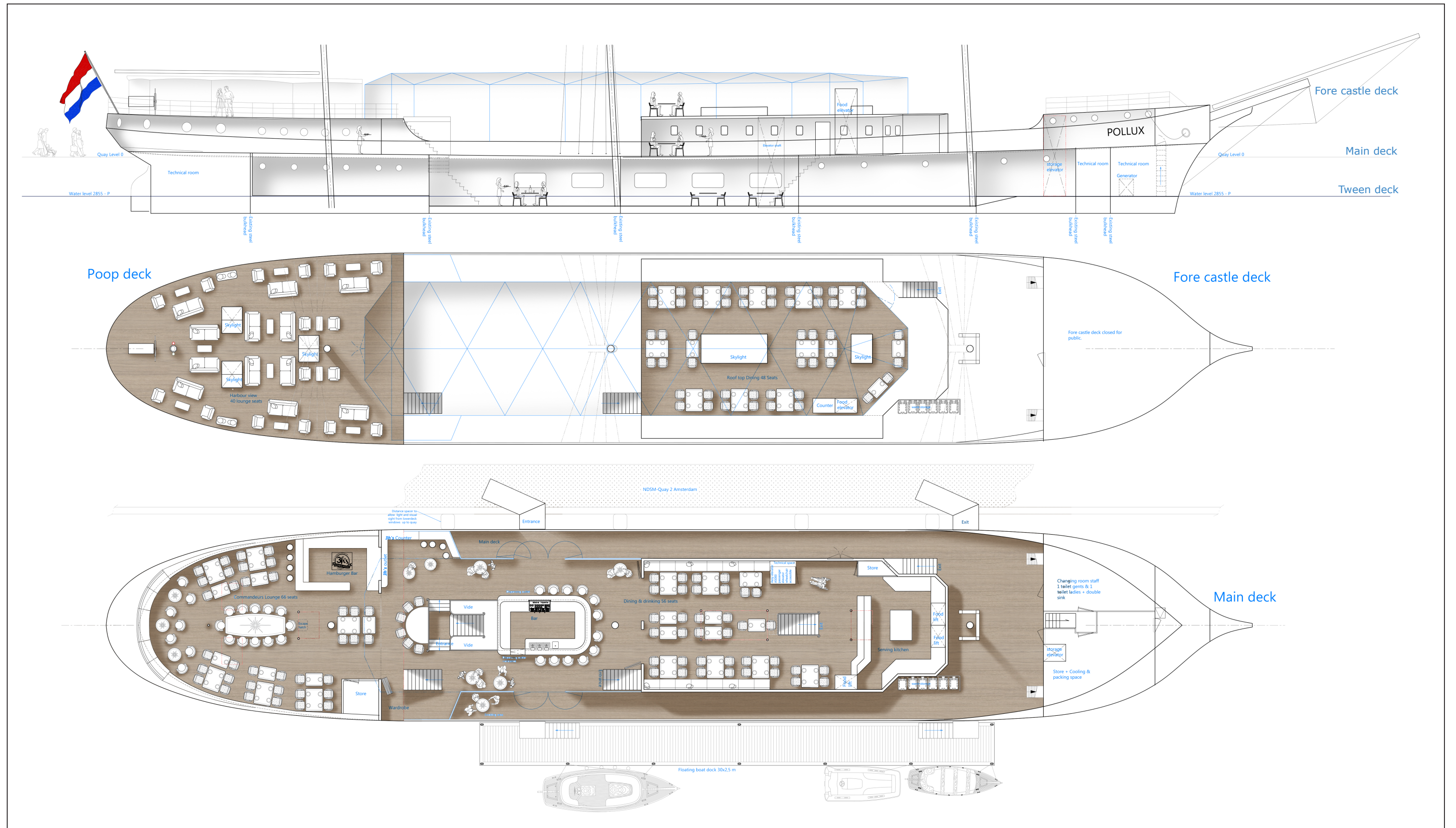
General arrangement
